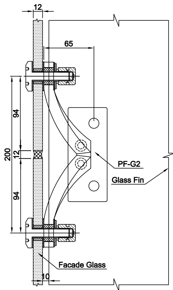
PF-G2 FIXING DETAIL
