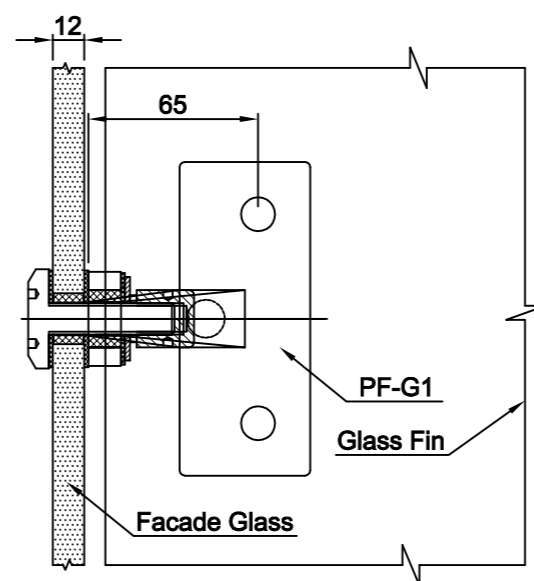
PF-G1 FIXING DETAIL
