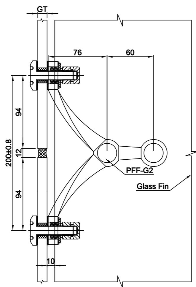
PFF-G2 FIXING DETAIL
