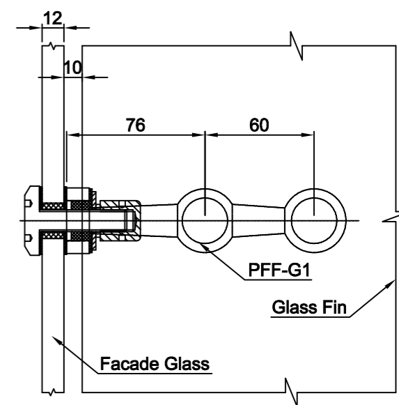
PFF-G1 FIXING DETAIL
